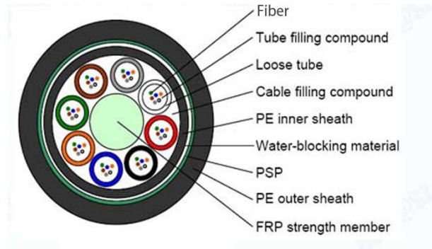
Cable Structure Diagram
