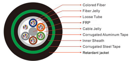
Cable Structure Diagram
